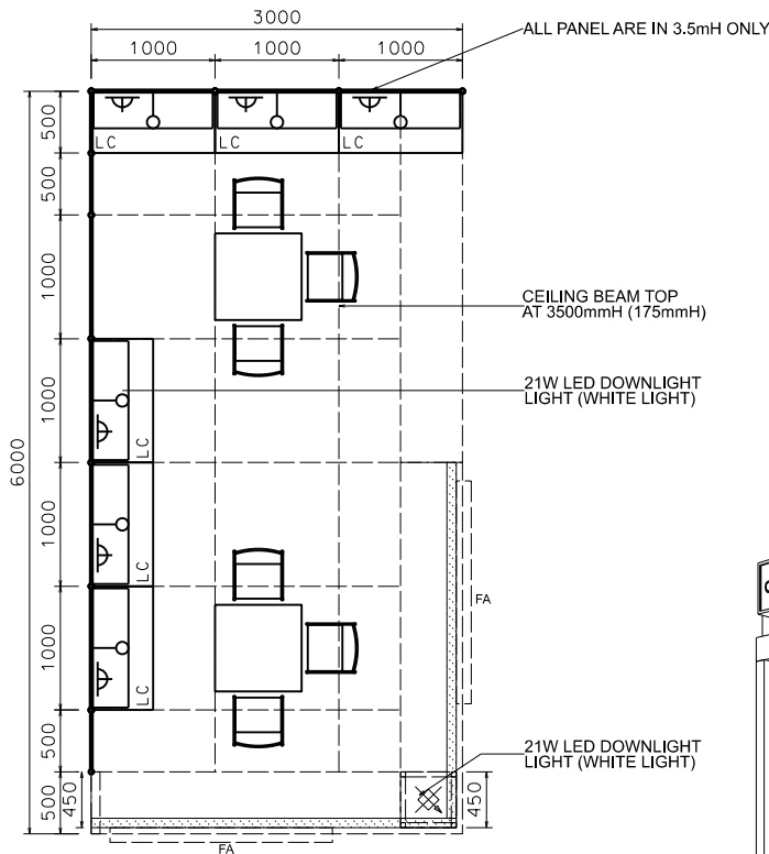
PLAN
